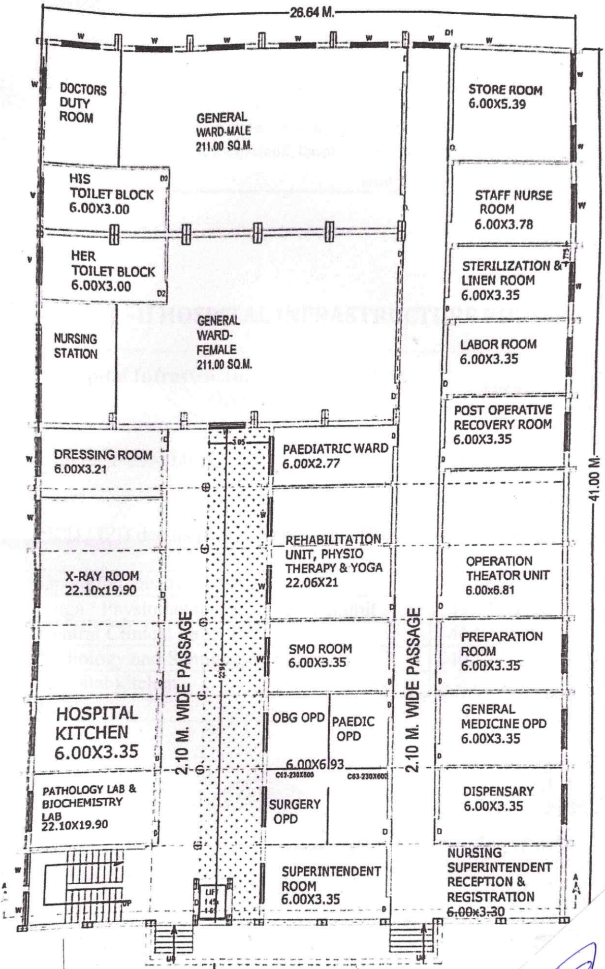
GROUND FLOOR PLAN (HOSI)
